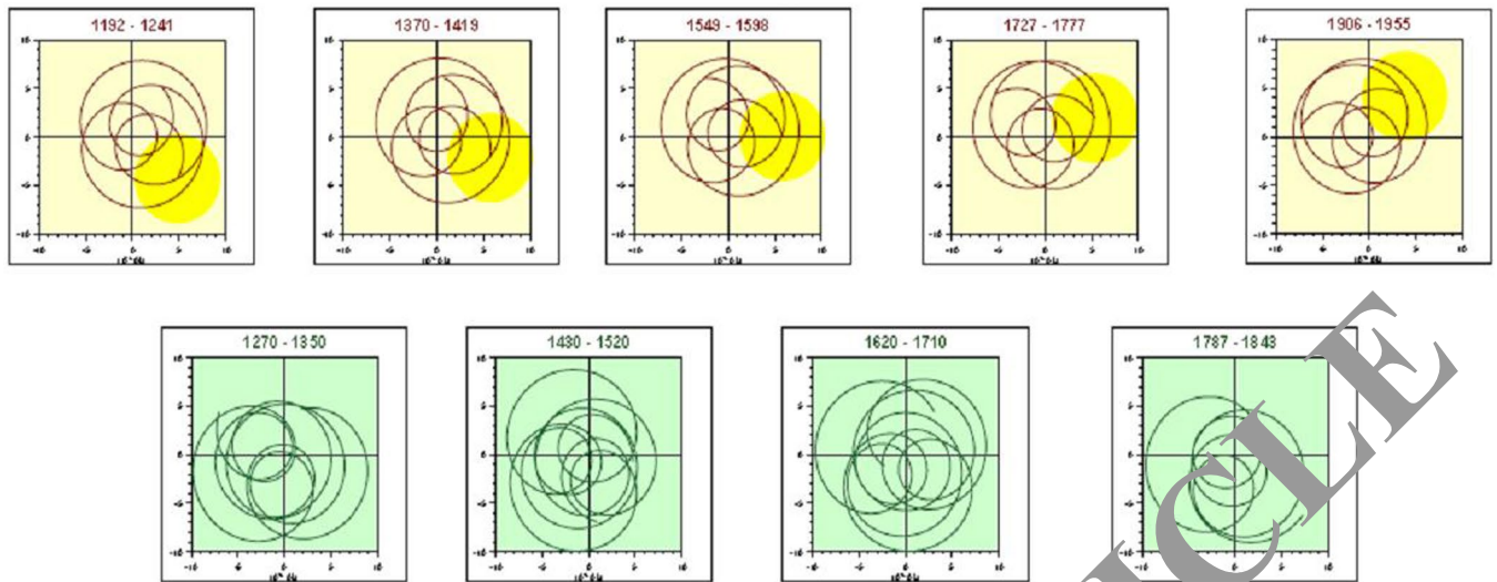
Figure 5. Schematic presentation of the solar inertial motion (SIM) about the barycenter of the solar system defined by the gravitational forces of large planets in the plane of ecliptic (the top plane in Fig. 4) for different time intervals shown in the top of each sub-figure (reproduced from Charvatova 36 ). The location of the Sun at the end of the period is shown by the yellow circles. Top row represent the ordered SIM affected by symmetric positions of large planets with respect to the Sun, while the bottom row shows the disorganized SIM with more random positions of large planets.
